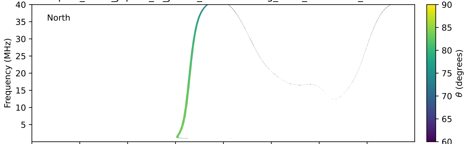
expres_earth_jupiter_io_jrm33_lossc-wid1deg_3kev_20220115_v11.cdf
