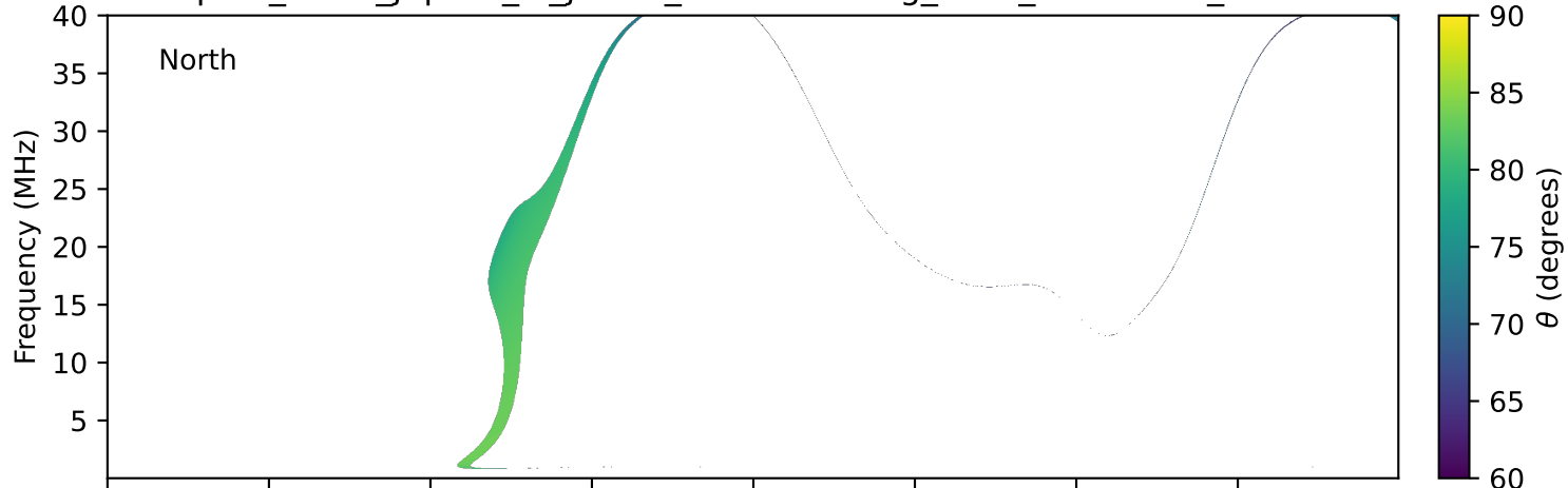
expres_earth_jupiter_io_jrm33_lossc-wid1deg_3kev_20220108_v11.cdf
