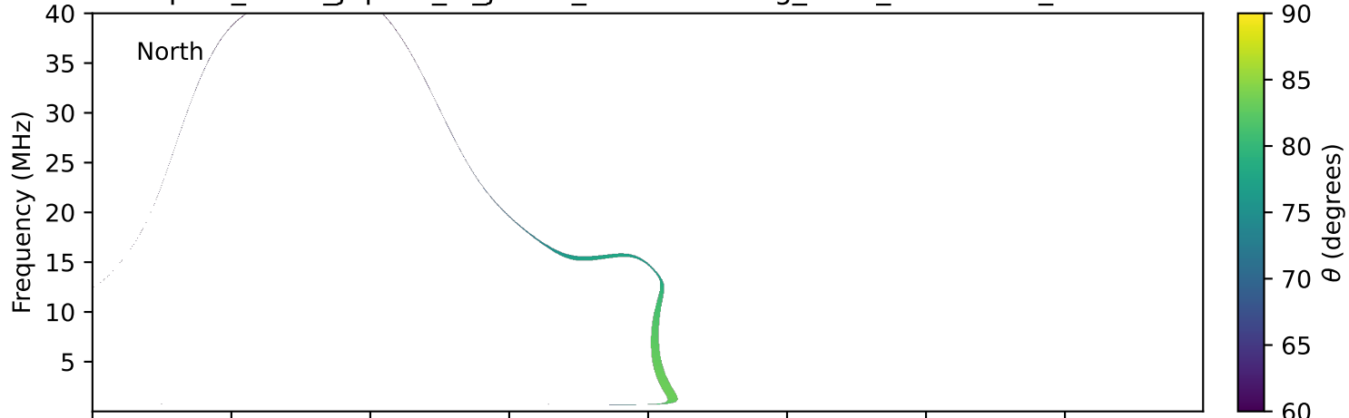
expres_earth_jupiter_io_jrm33_lossc-wid1deg_3kev_20220105_v11.cdf
