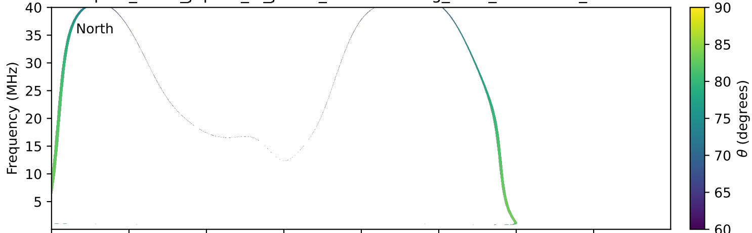
expres_earth_jupiter_io_jrm33_lossc-wid1deg_3kev_20220103_v11.cdf
