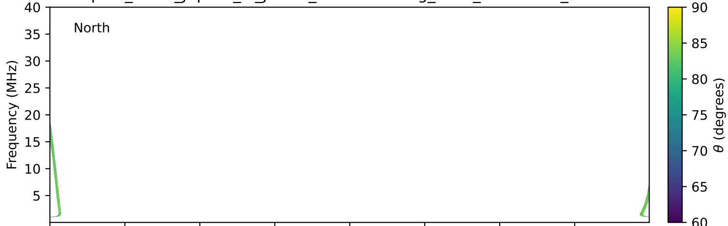
expres_earth_jupiter_io_jrm33_lossc-wid1deg_3kev_20220102_v11.cdf
