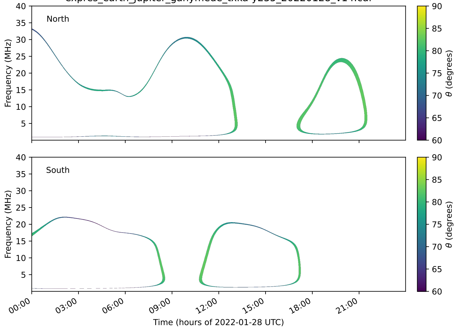
expres_earth_jupiter_ganymede_txka-y235_20220128_v14.cdf
