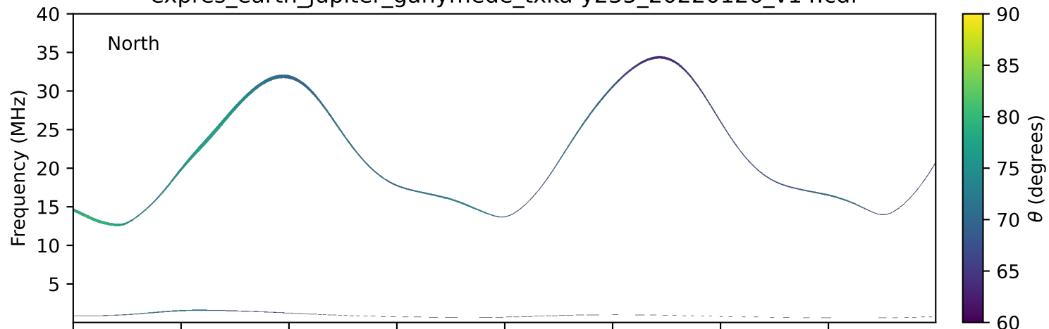
expres_earth_jupiter_ganymede_txka-y235_20220126_v14.cdf
