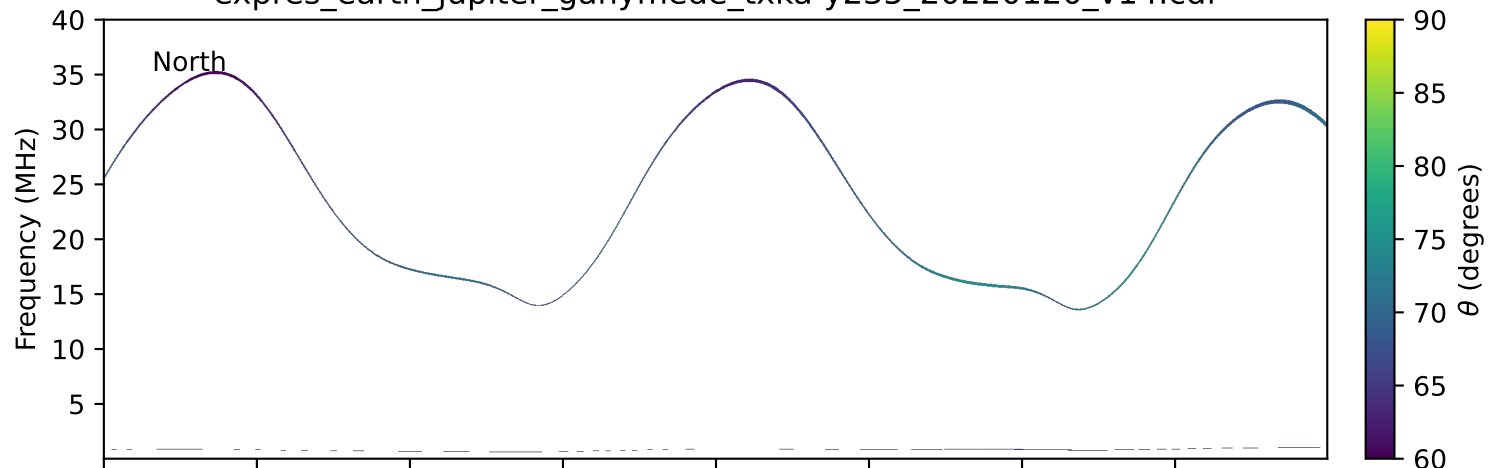
expres_earth_jupiter_ganymede_txka-y235_20220120_v14.cdf
