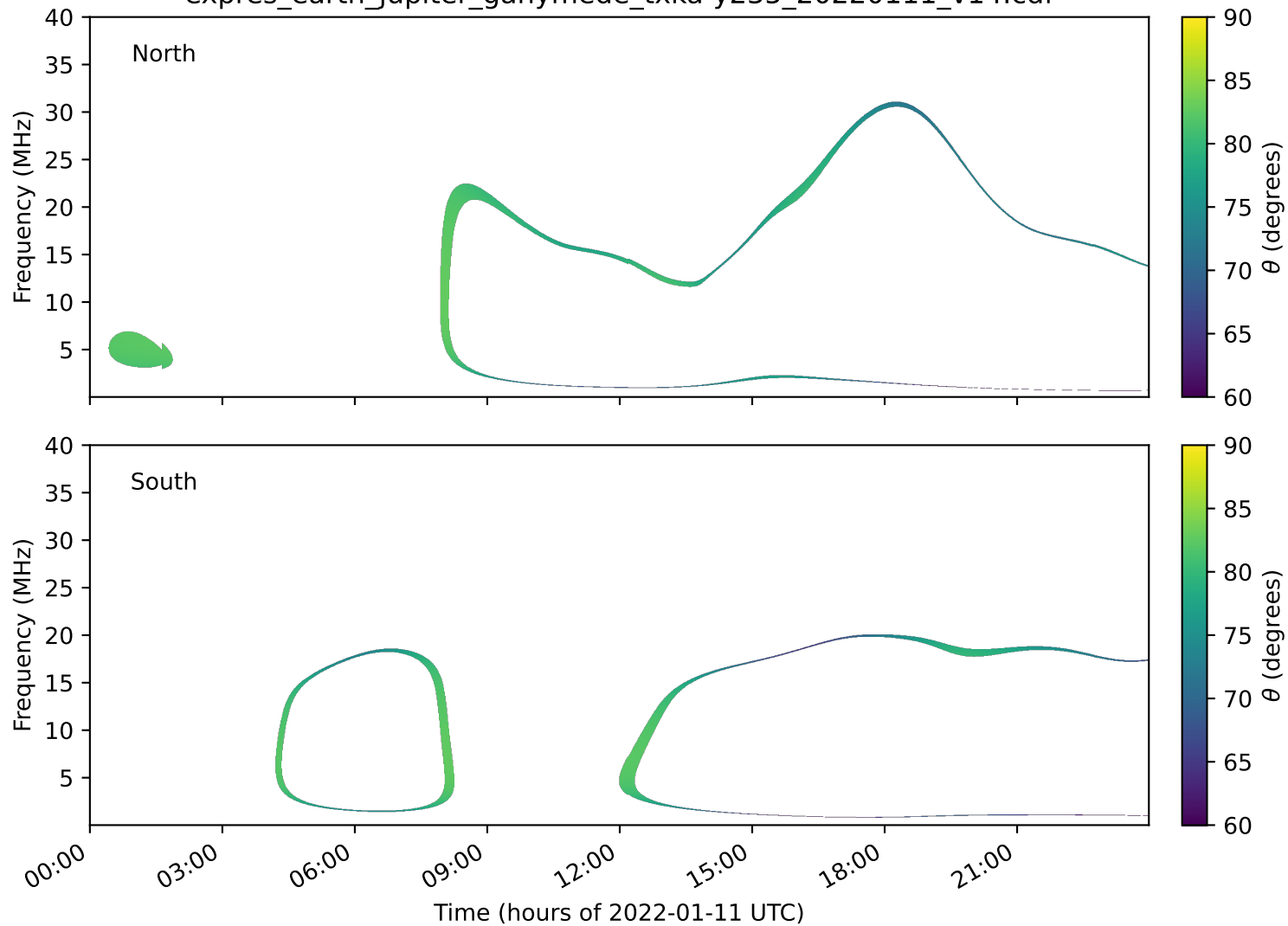
expres_earth_jupiter_ganymede_txka-y235_20220111_v14.cdf
