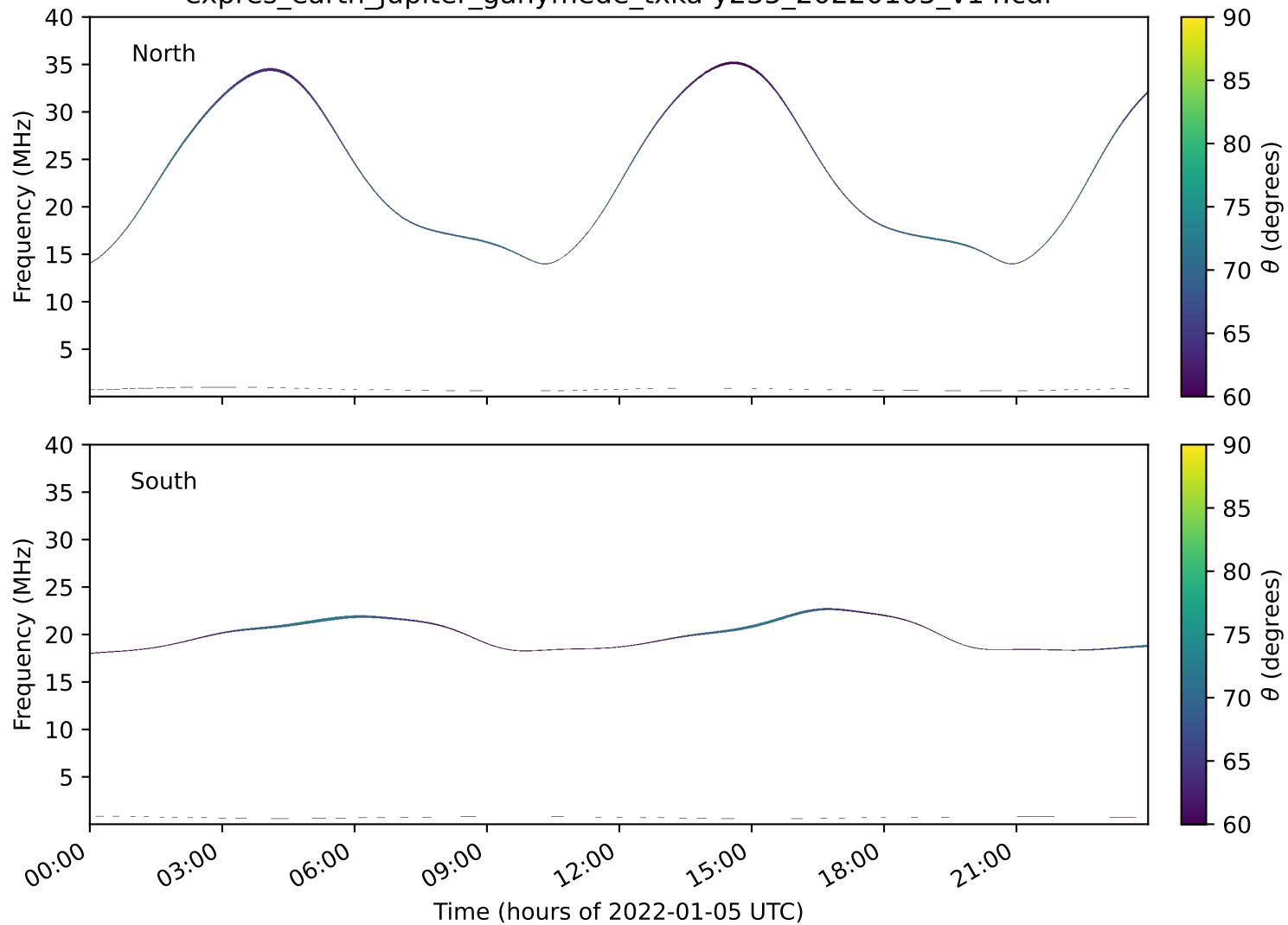
expres_earth_jupiter_ganymede_txka-y235_20220105_v14.cdf
