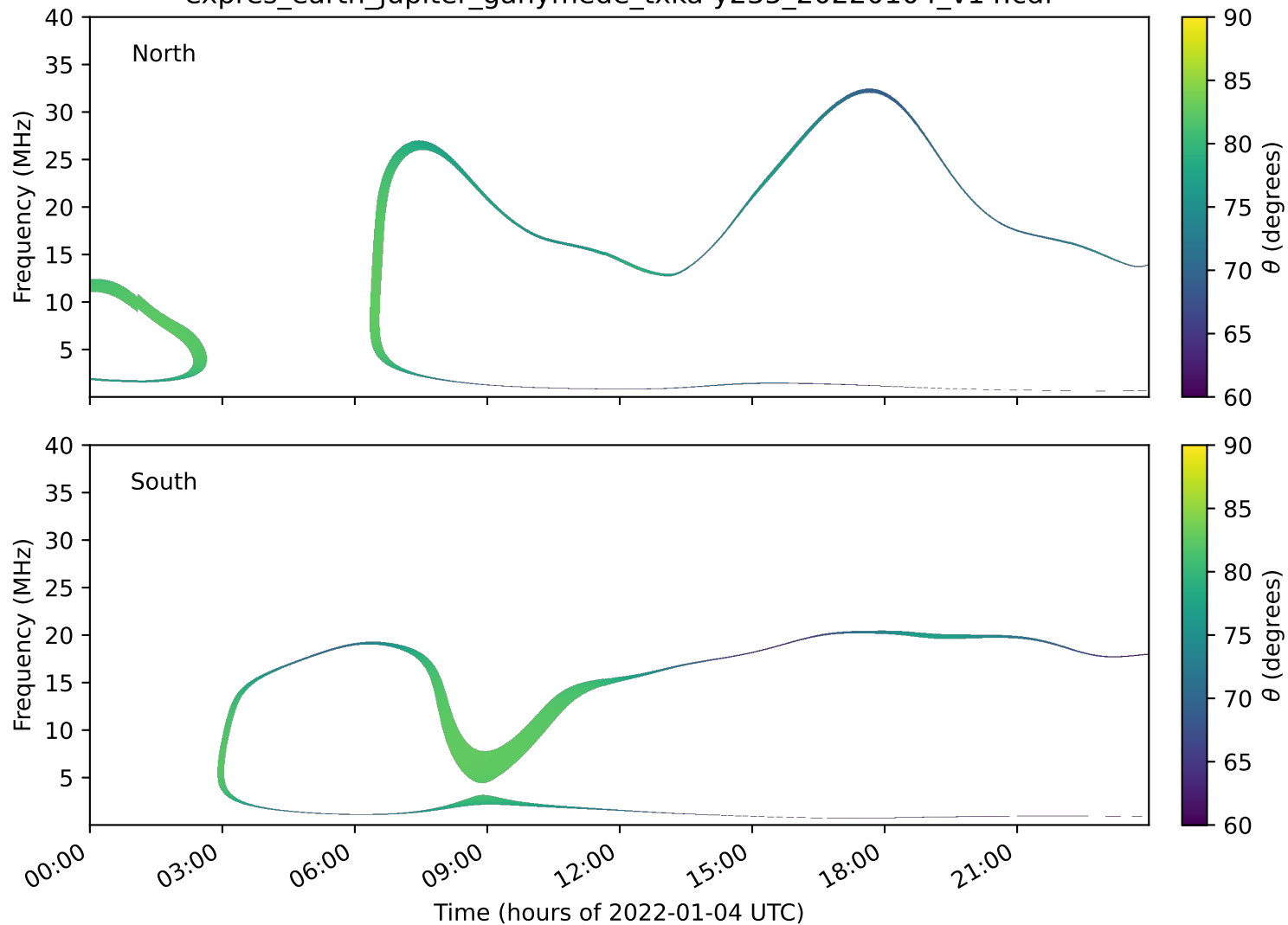
expres_earth_jupiter_ganymede_txka-y235_20220104_v14.cdf
