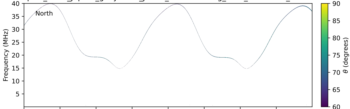
expres_earth_jupiter_ganymede_jrm33_lossc-wid1deg_3kev_20220120_v11.cdf
