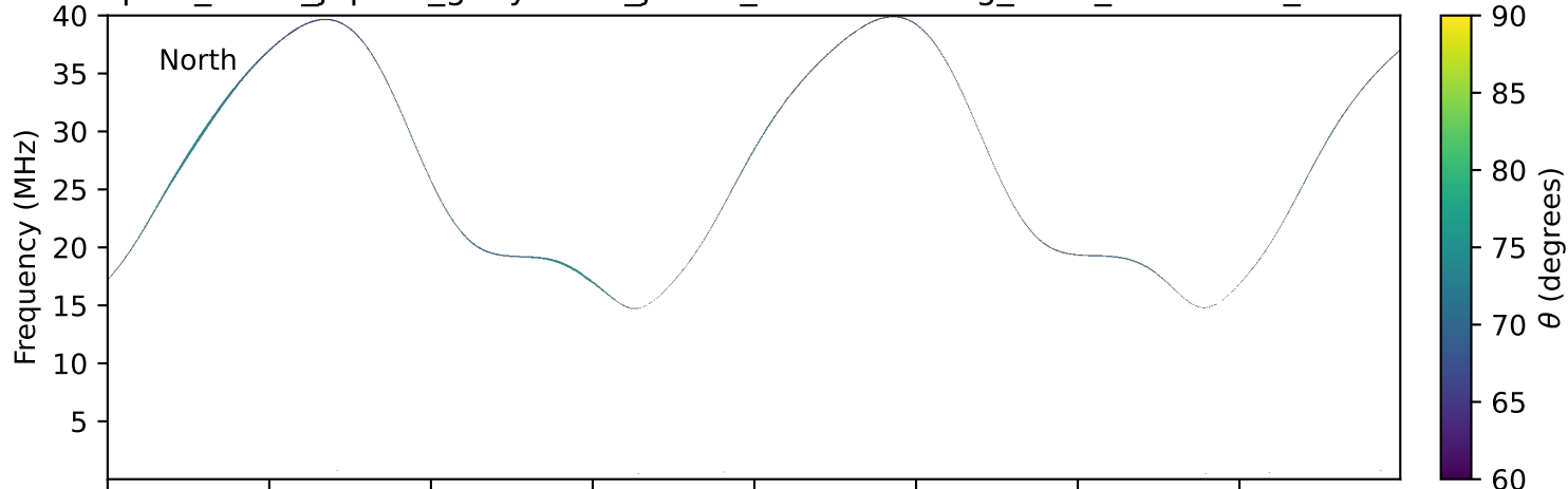
expres_earth_jupiter_ganymede_jrm33_lossc-wid1deg_3kev_20220105_v11.cdf
