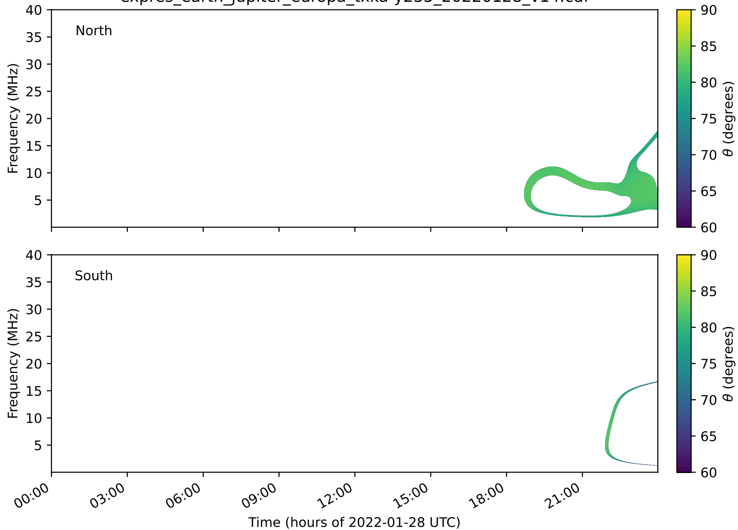
expres_earth_jupiter_europa_txka-y235_20220128_v14.cdf
