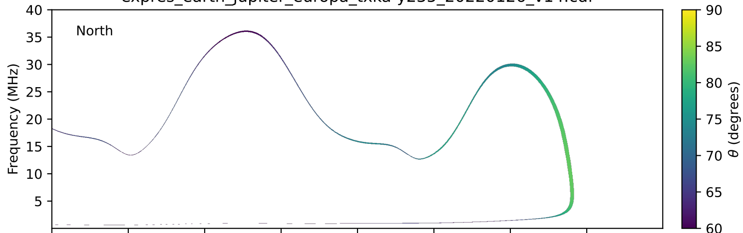
expres_earth_jupiter_europa_txka-y235_20220126_v14.cdf
