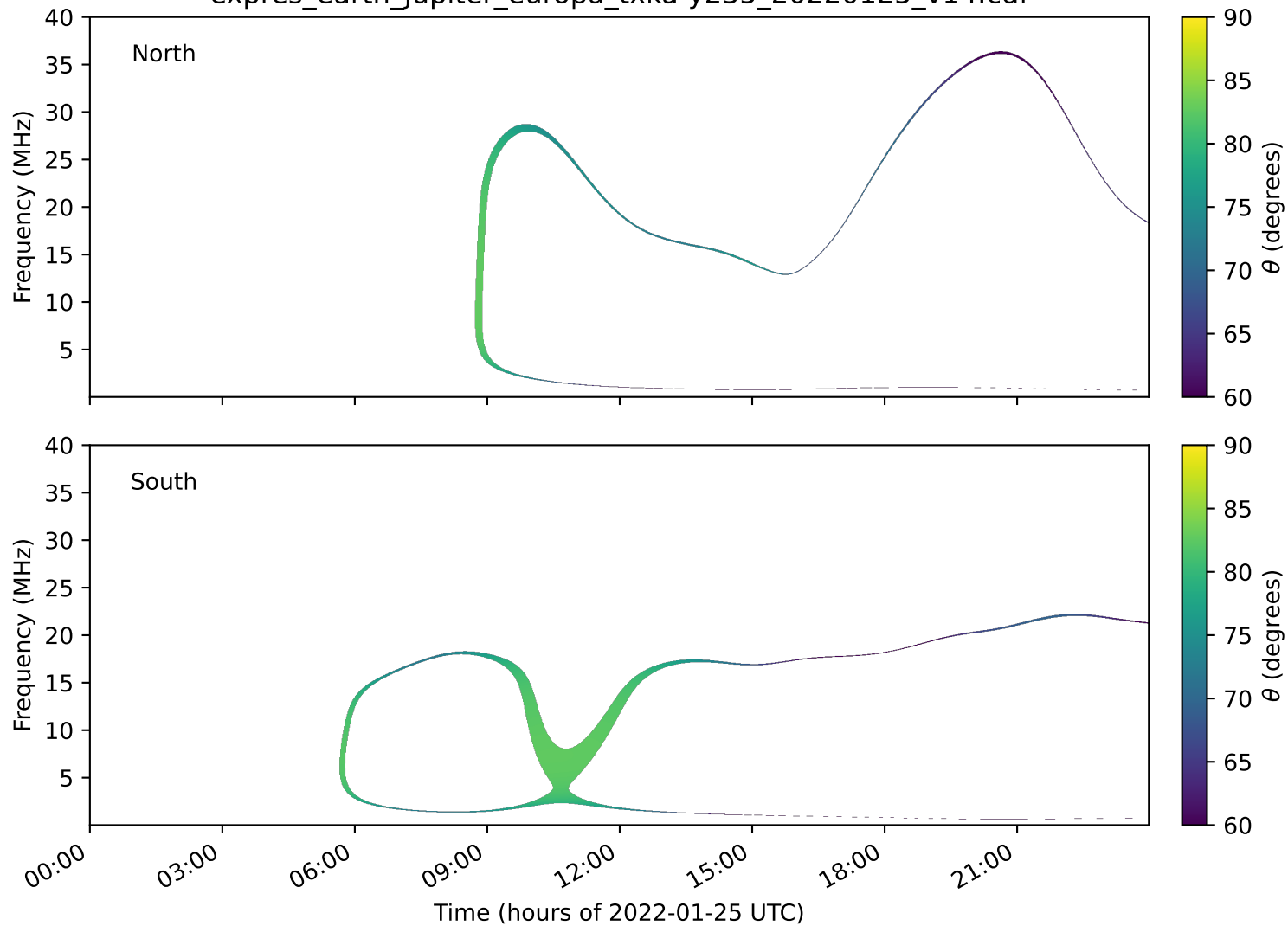
expres_earth_jupiter_europa_txka-y235_20220125_v14.cdf
