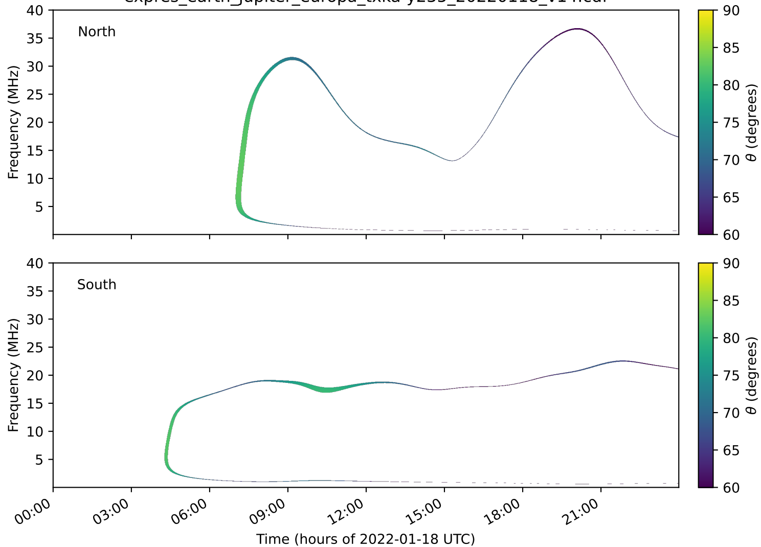
expres_earth_jupiter_europa_txka-y235_20220118_v14.cdf
