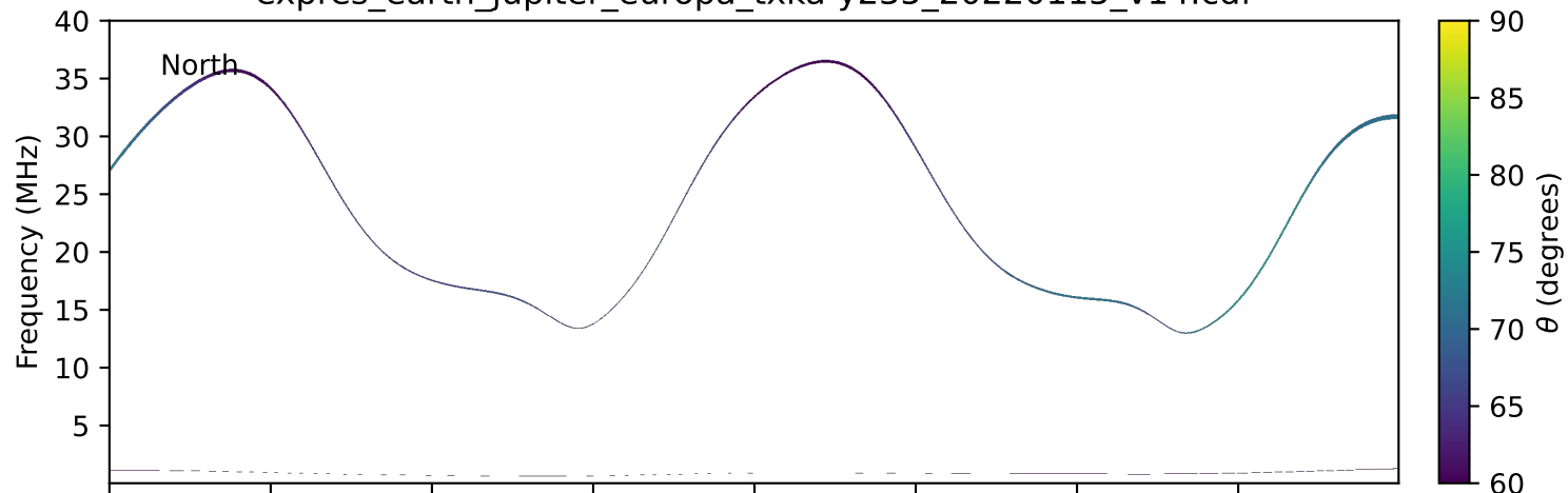
expres_earth_jupiter_europa_txka-y235_20220115_v14.cdf
