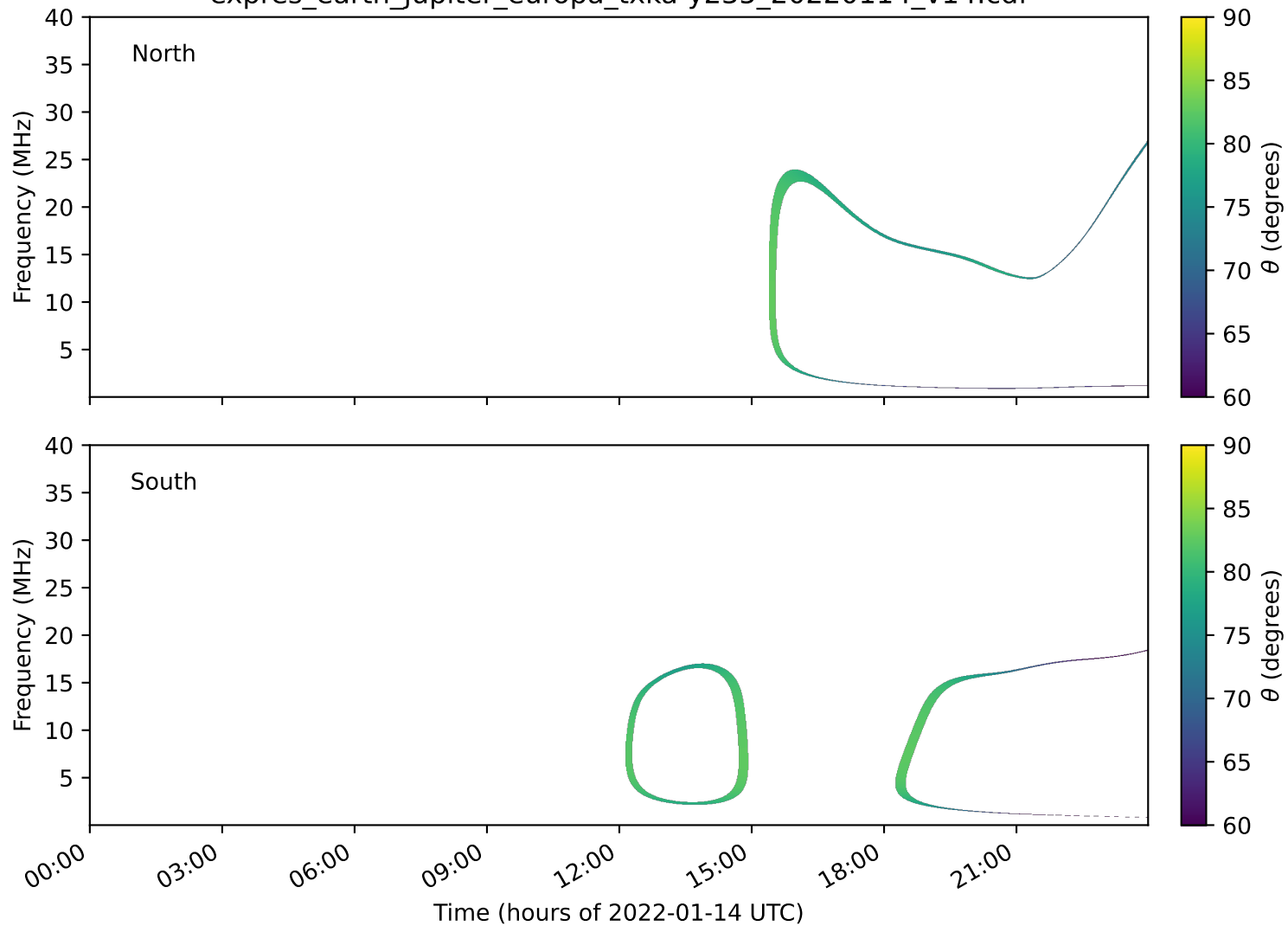
expres_earth_jupiter_europa_txka-y235_20220114_v14.cdf
