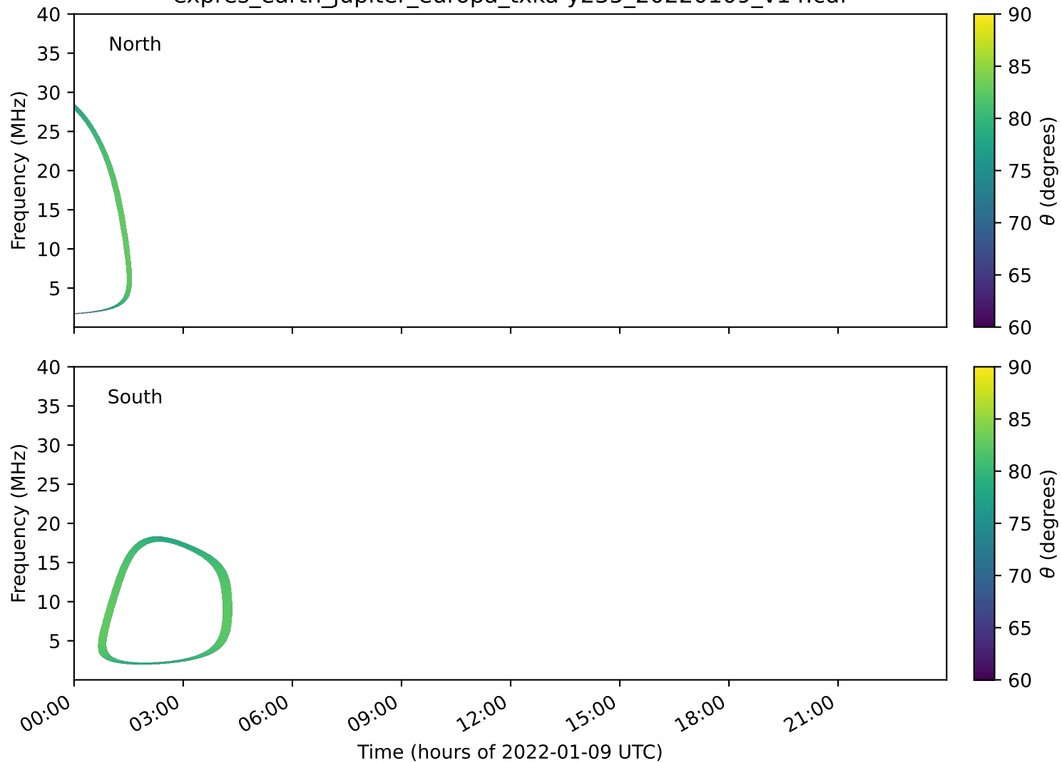
expres_earth_jupiter_europa_txka-y235_20220109_v14.cdf
