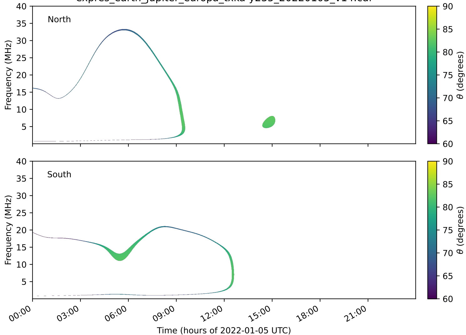
expres_earth_jupiter_europa_txka-y235_20220105_v14.cdf
