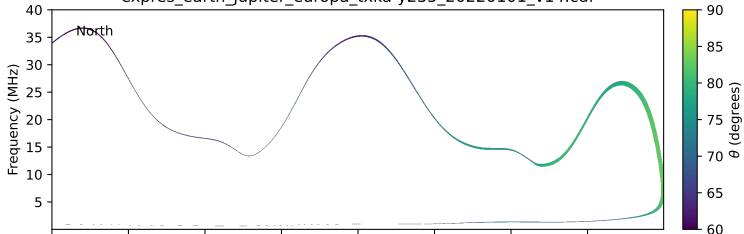
expres_earth_jupiter_europa_txka-y235_20220101_v14.cdf
