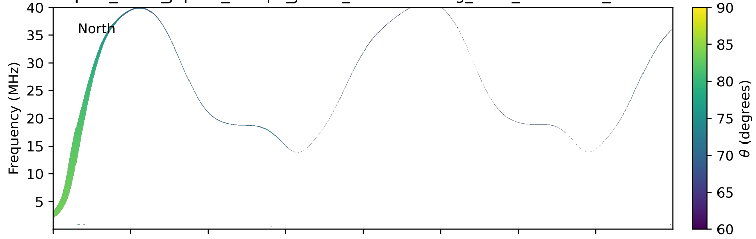
expres_earth_jupiter_europa_jrm33_lossc-wid1deg_3kev_20220129_v11.cdf
