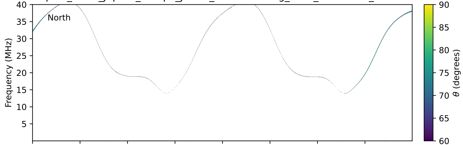
expres_earth_jupiter_europa_jrm33_lossc-wid1deg_3kev_20220115_v11.cdf
