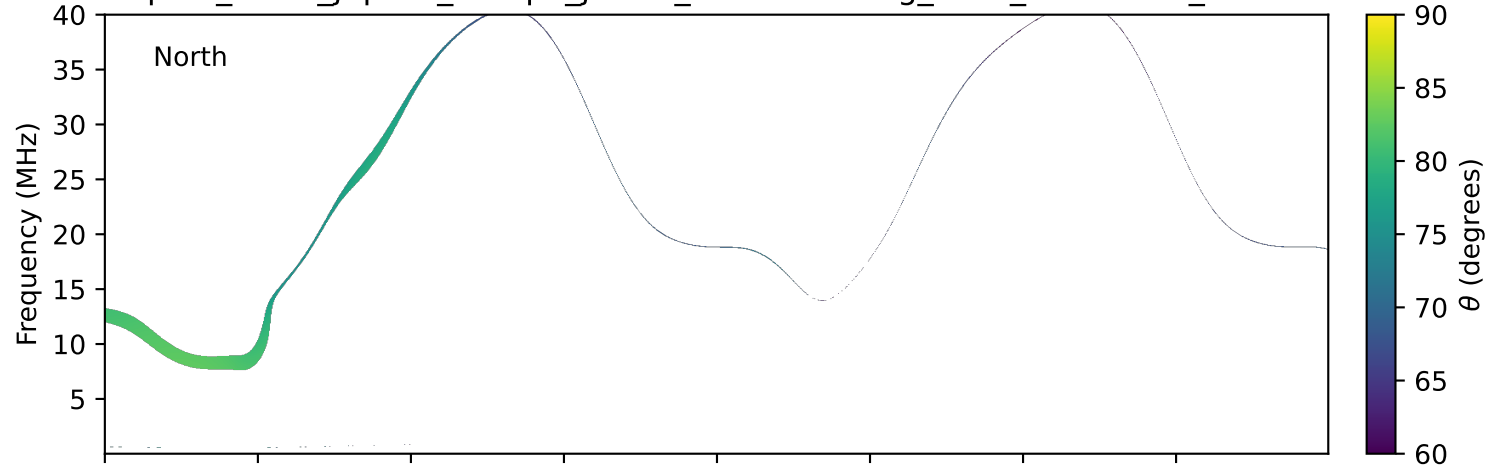
expres_earth_jupiter_europa_jrm33_lossc-wid1deg_3kev_20220104_v11.cdf
