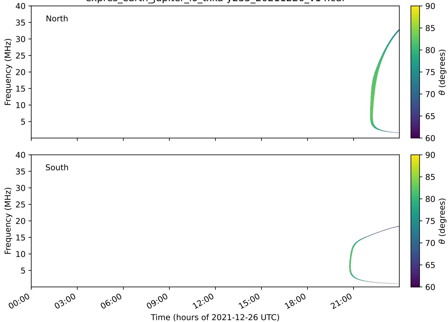
expres_earth_jupiter_io_txka-y235_20211226_v14.cdf
