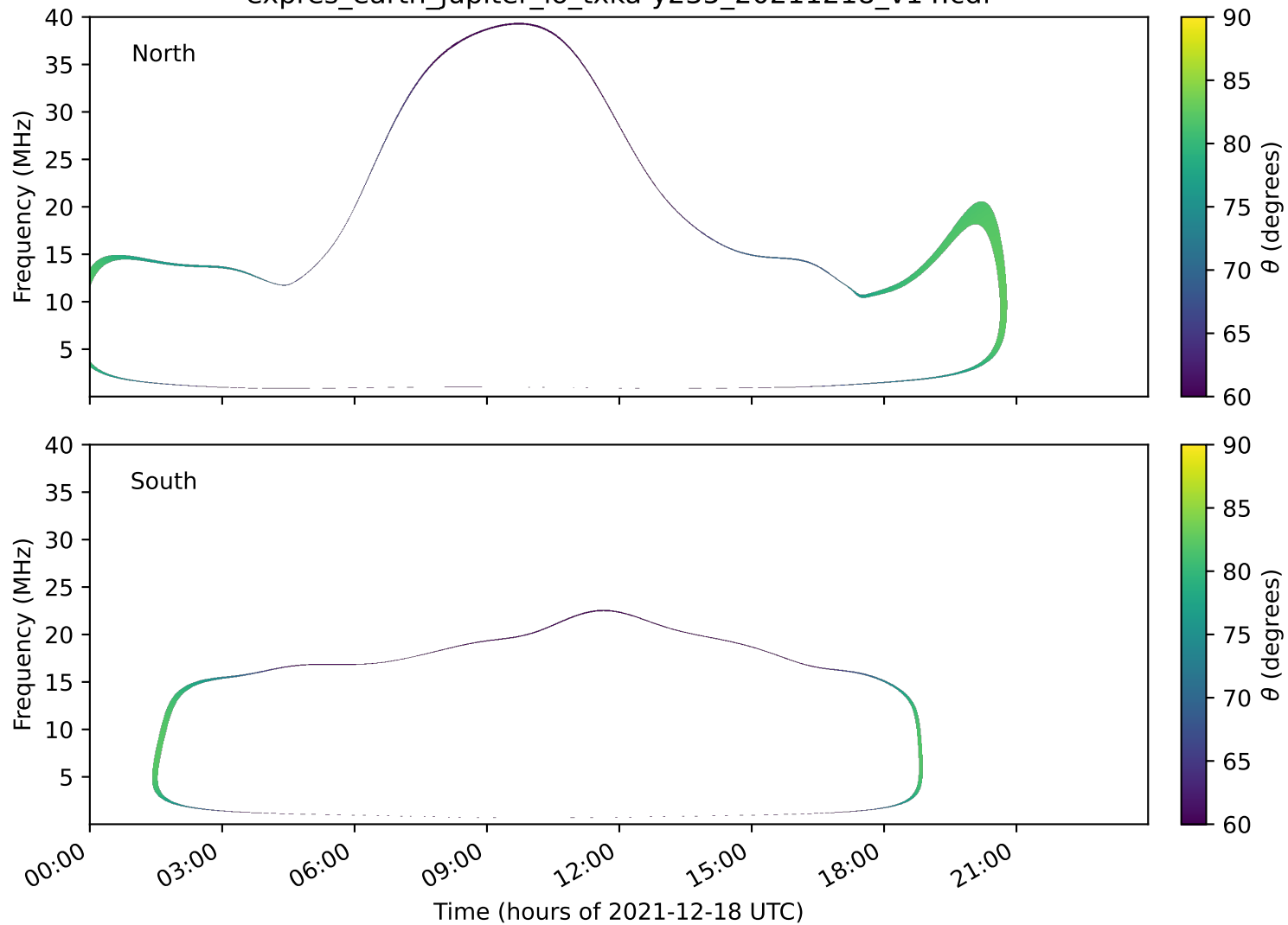
expres_earth_jupiter_io_txka-y235_20211218_v14.cdf
