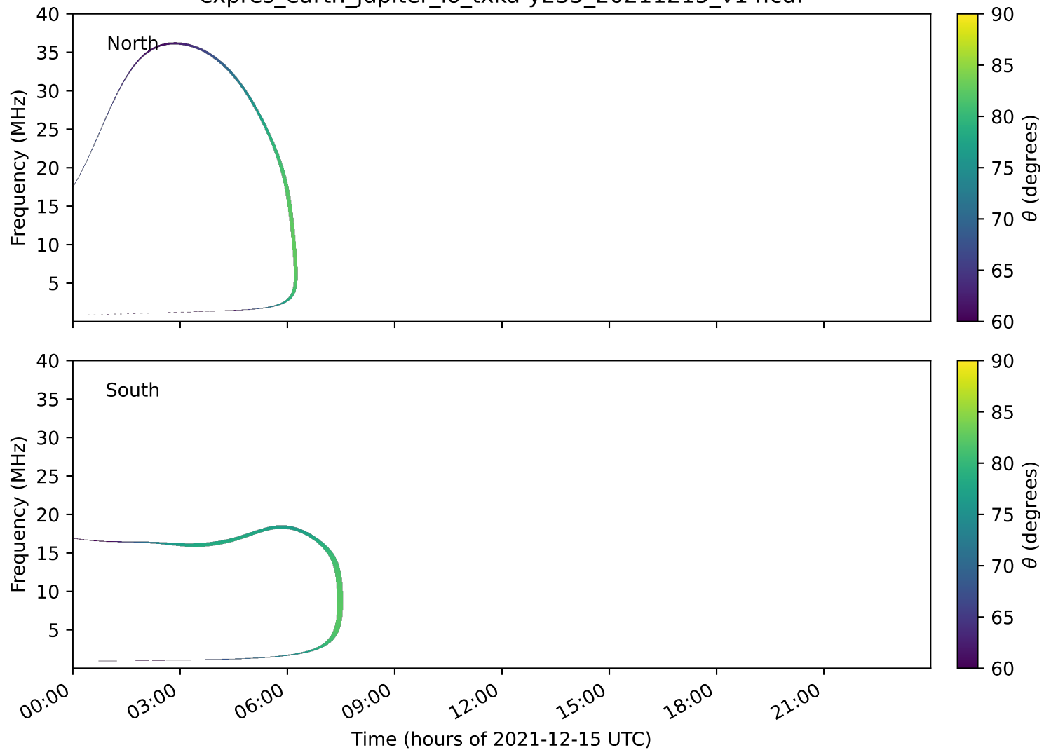
expres_earth_jupiter_io_txka-y235_20211215_v14.cdf
