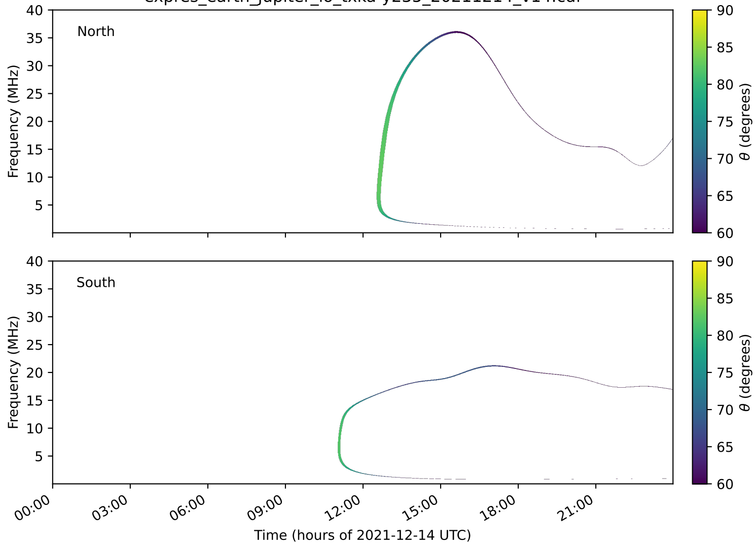
expres_earth_jupiter_io_txka-y235_20211214_v14.cdf
