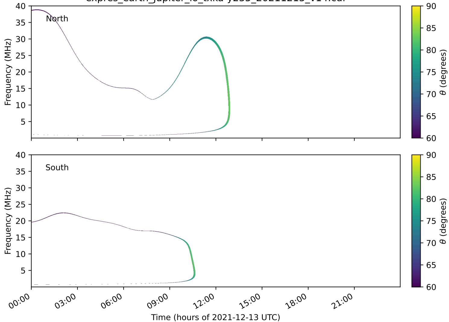
expres_earth_jupiter_io_txka-y235_20211213_v14.cdf
