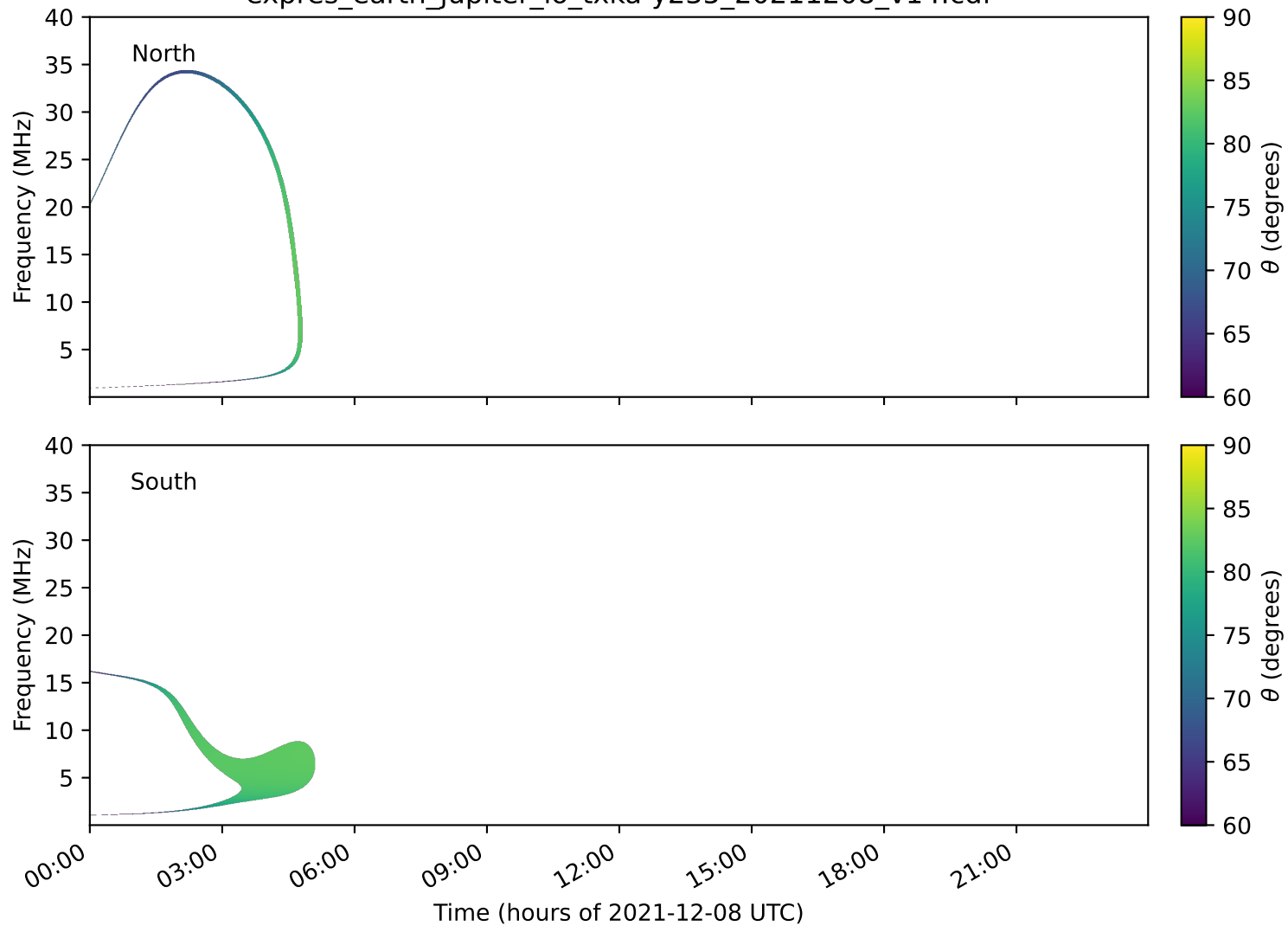
expres_earth_jupiter_io_txka-y235_20211208_v14.cdf
