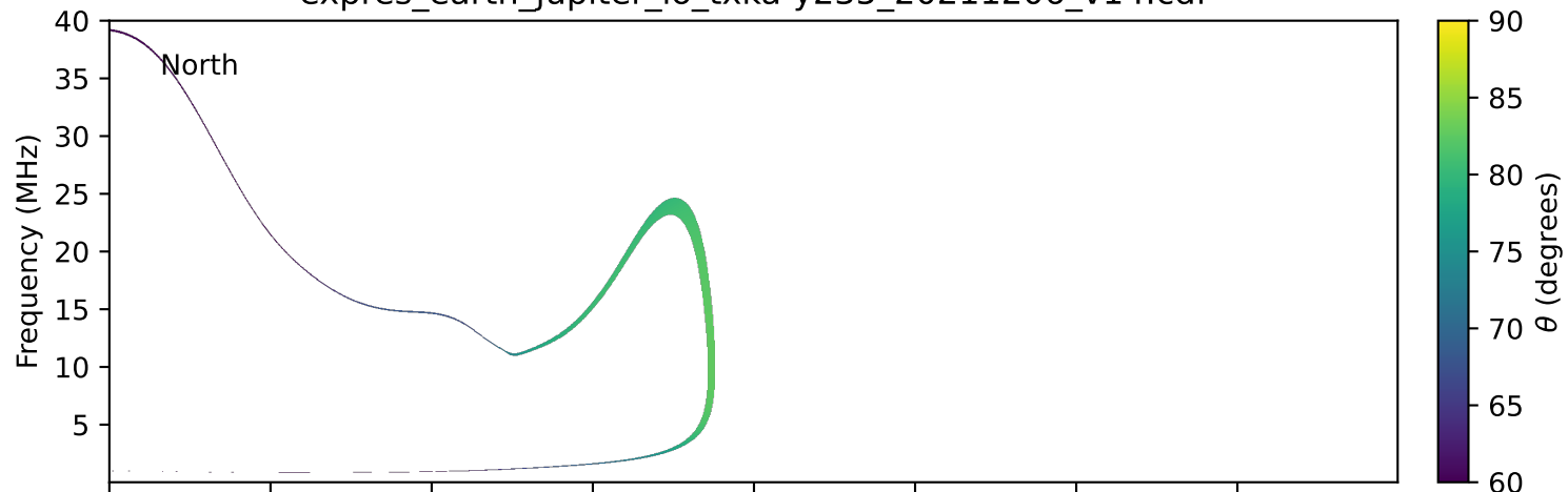
expres_earth_jupiter_io_txka-y235_20211206_v14.cdf
