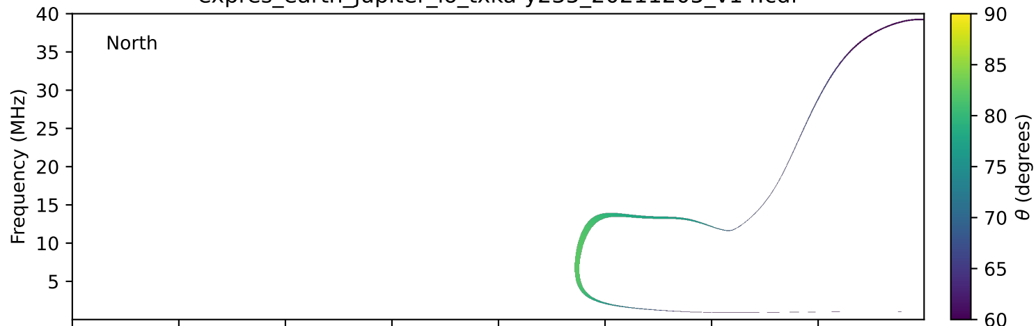
expres_earth_jupiter_io_txka-y235_20211205_v14.cdf
