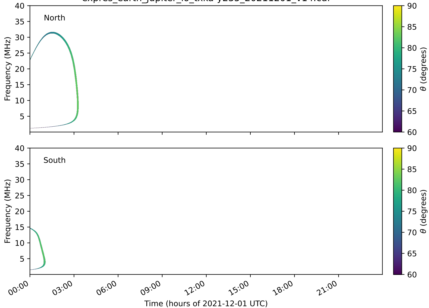
expres_earth_jupiter_io_txka-y235_20211201_v14.cdf
