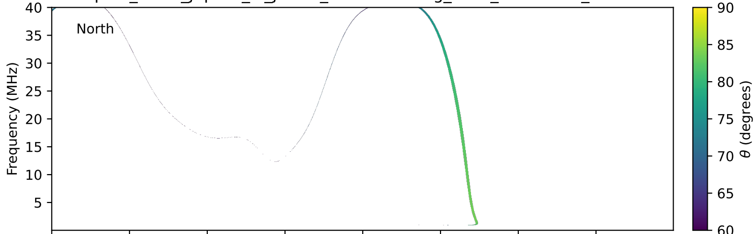
expres_earth_jupiter_io_jrm33_lossc-wid1deg_3kev_20211227_v11.cdf
