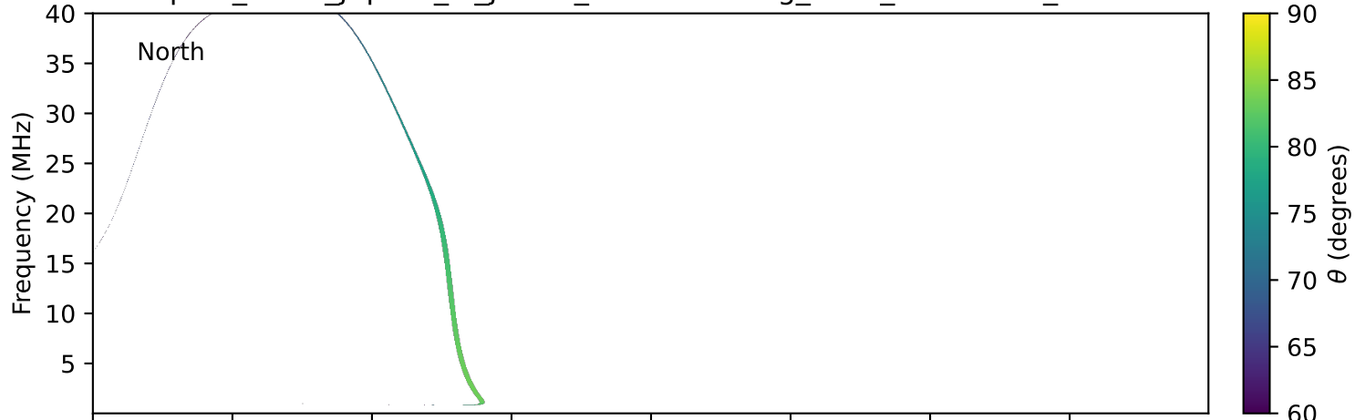
expres_earth_jupiter_io_jrm33_lossc-wid1deg_3kev_20211222_v11.cdf
