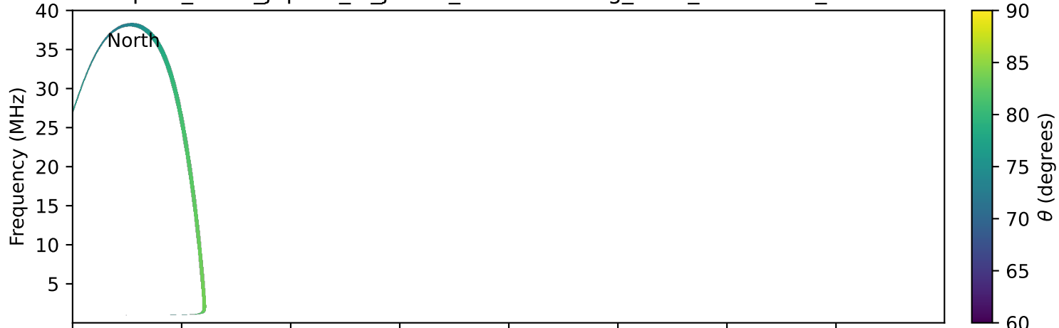
expres_earth_jupiter_io_jrm33_lossc-wid1deg_3kev_20211201_v11.cdf
