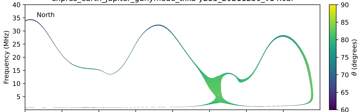
expres_earth_jupiter_ganymede_txka-y235_20211230_v14.cdf
