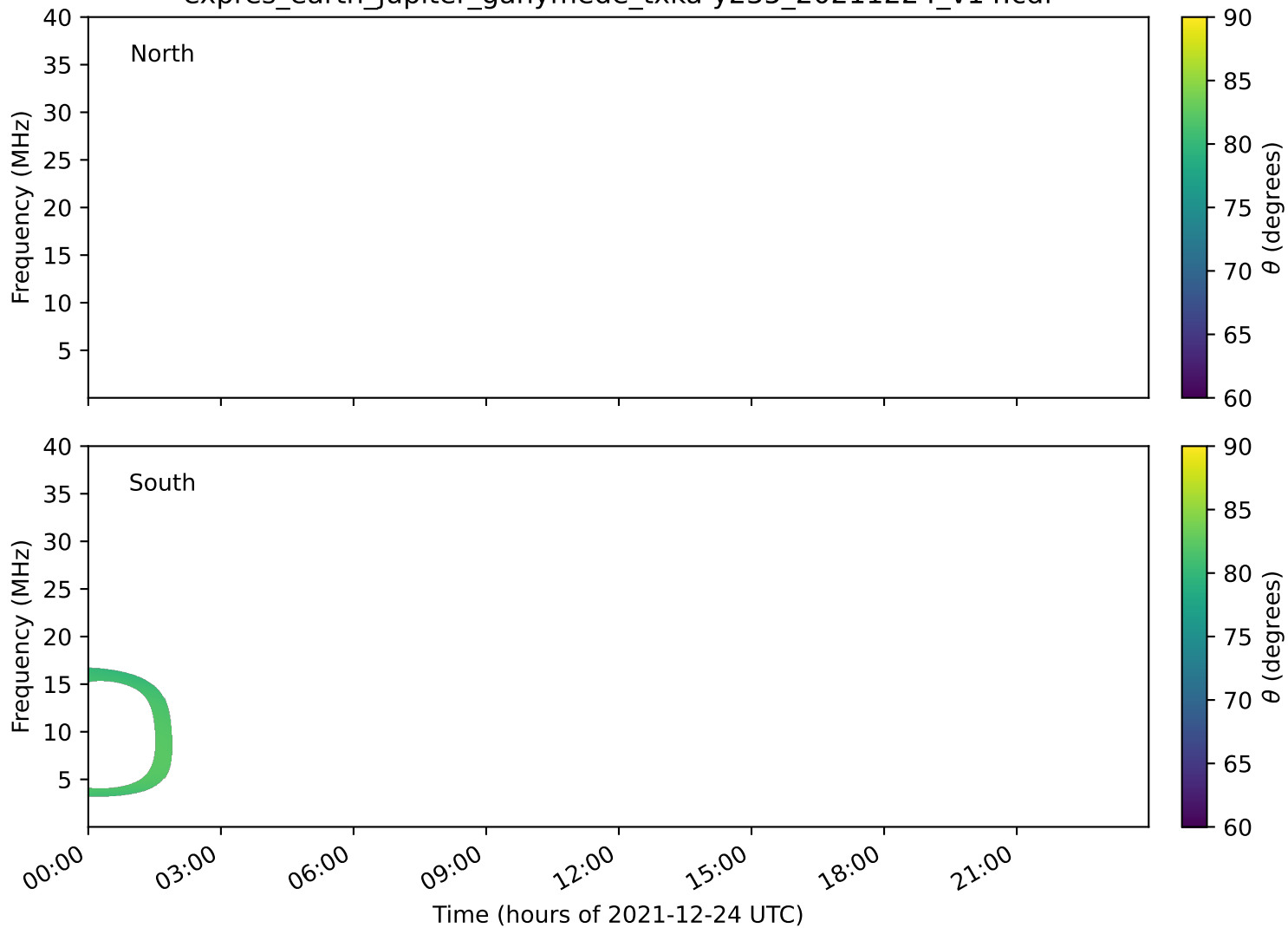
expres_earth_jupiter_ganymede_txka-y235_20211224_v14.cdf
