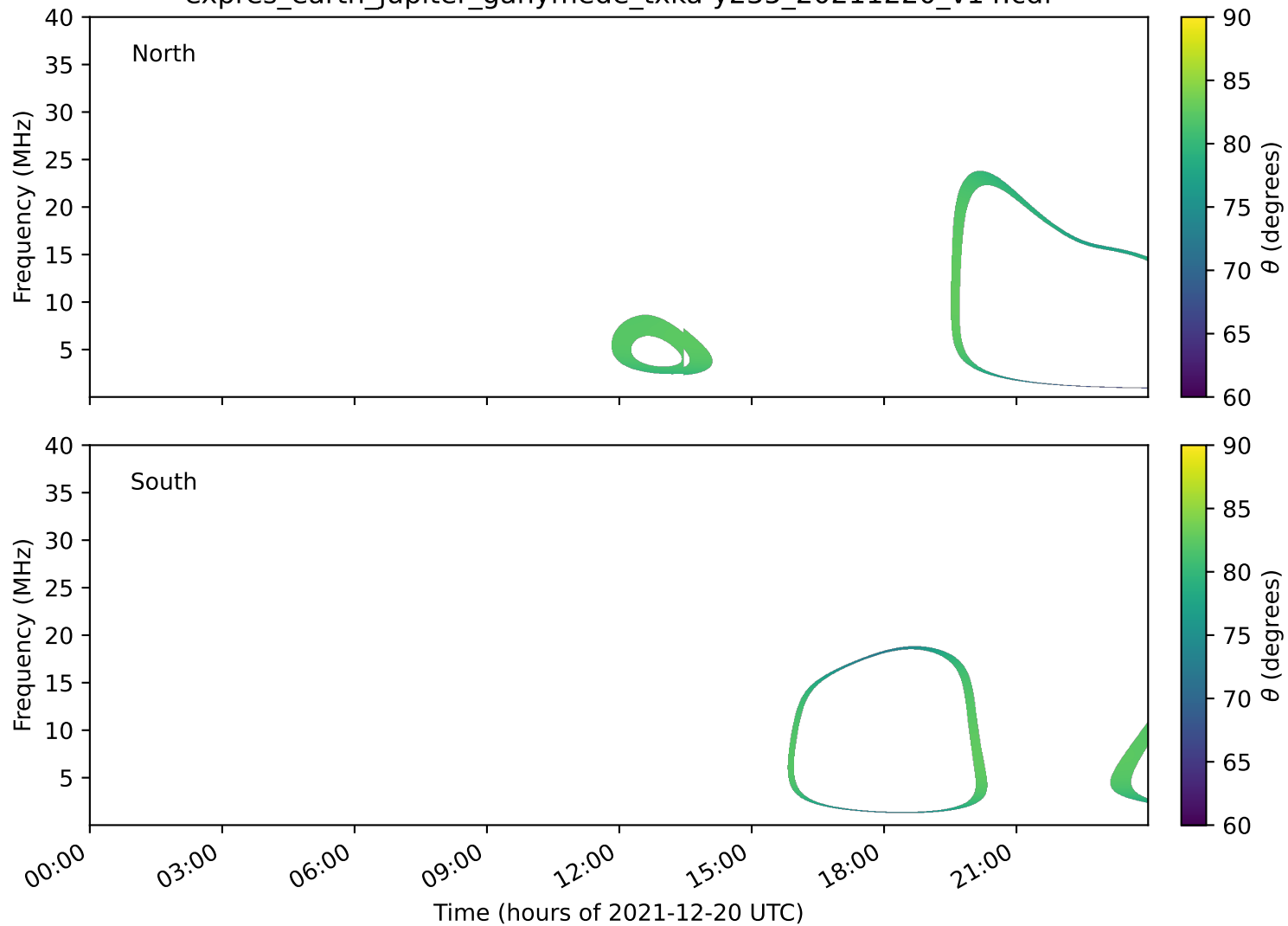
expres_earth_jupiter_ganymede_txka-y235_20211220_v14.cdf
