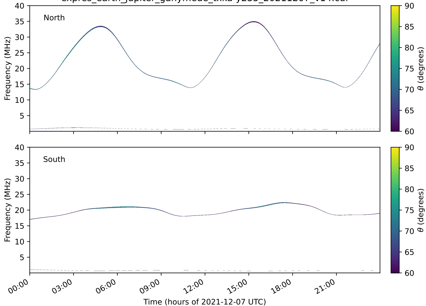
expres_earth_jupiter_ganymede_txka-y235_20211207_v14.cdf
