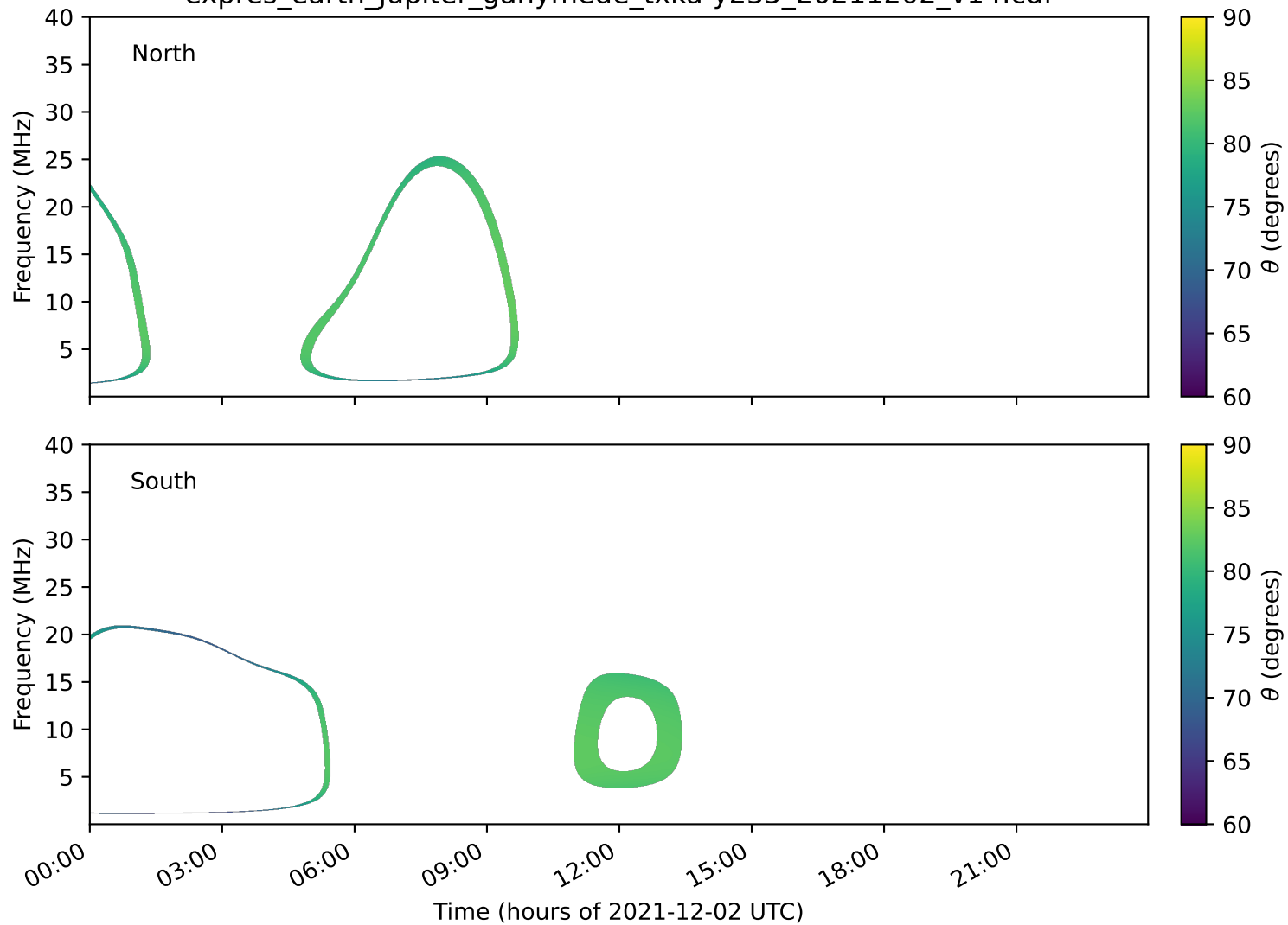
expres_earth_jupiter_ganymede_txka-y235_20211202_v14.cdf
