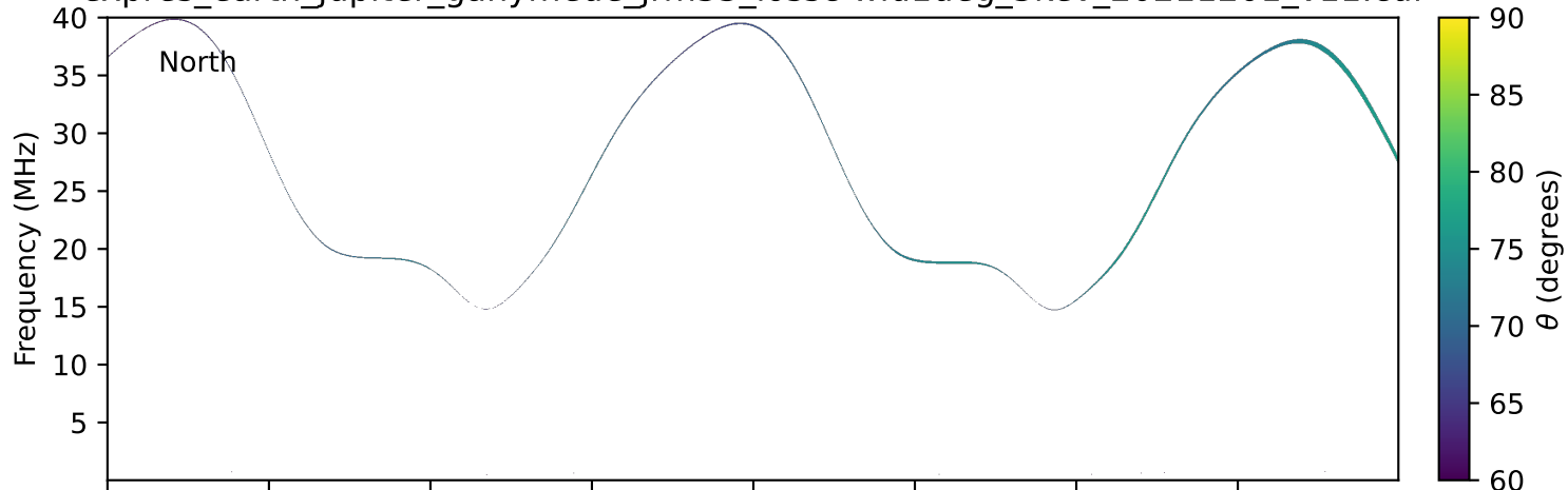
expres_earth_jupiter_ganymede_jrm33_lossc-wid1deg_3kev_20211201_v11.cdf
