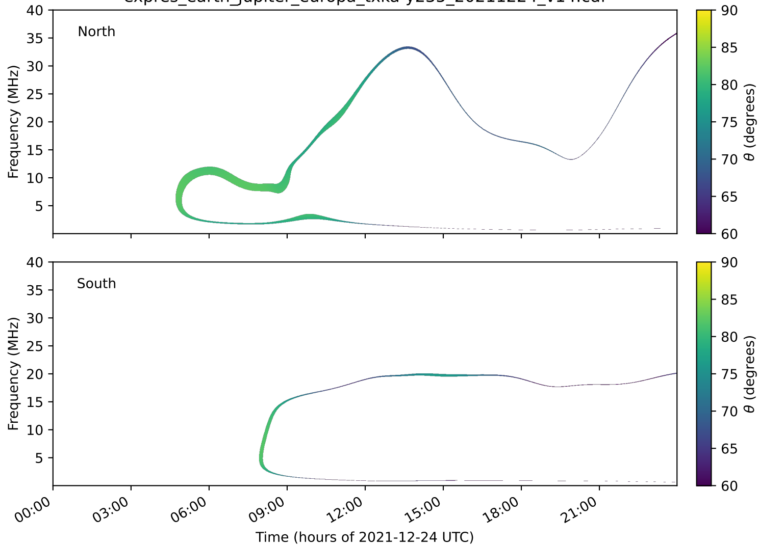
expres_earth_jupiter_europa_txka-y235_20211224_v14.cdf
