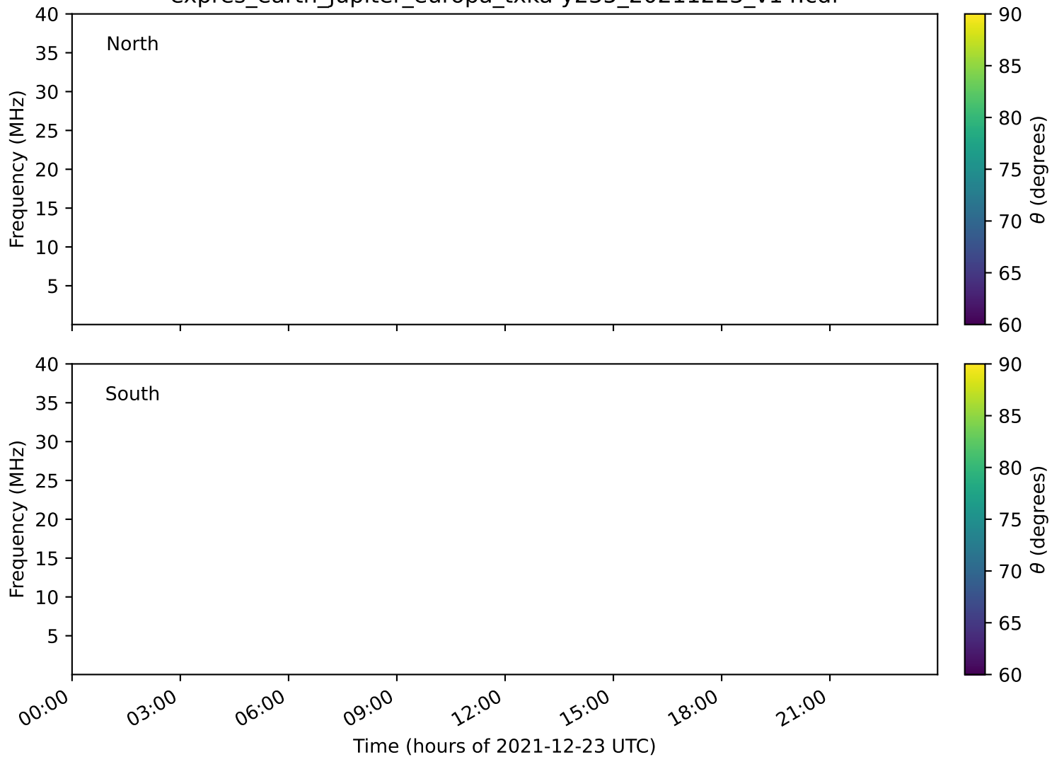
expres_earth_jupiter_europa_txka-y235_20211223_v14.cdf
