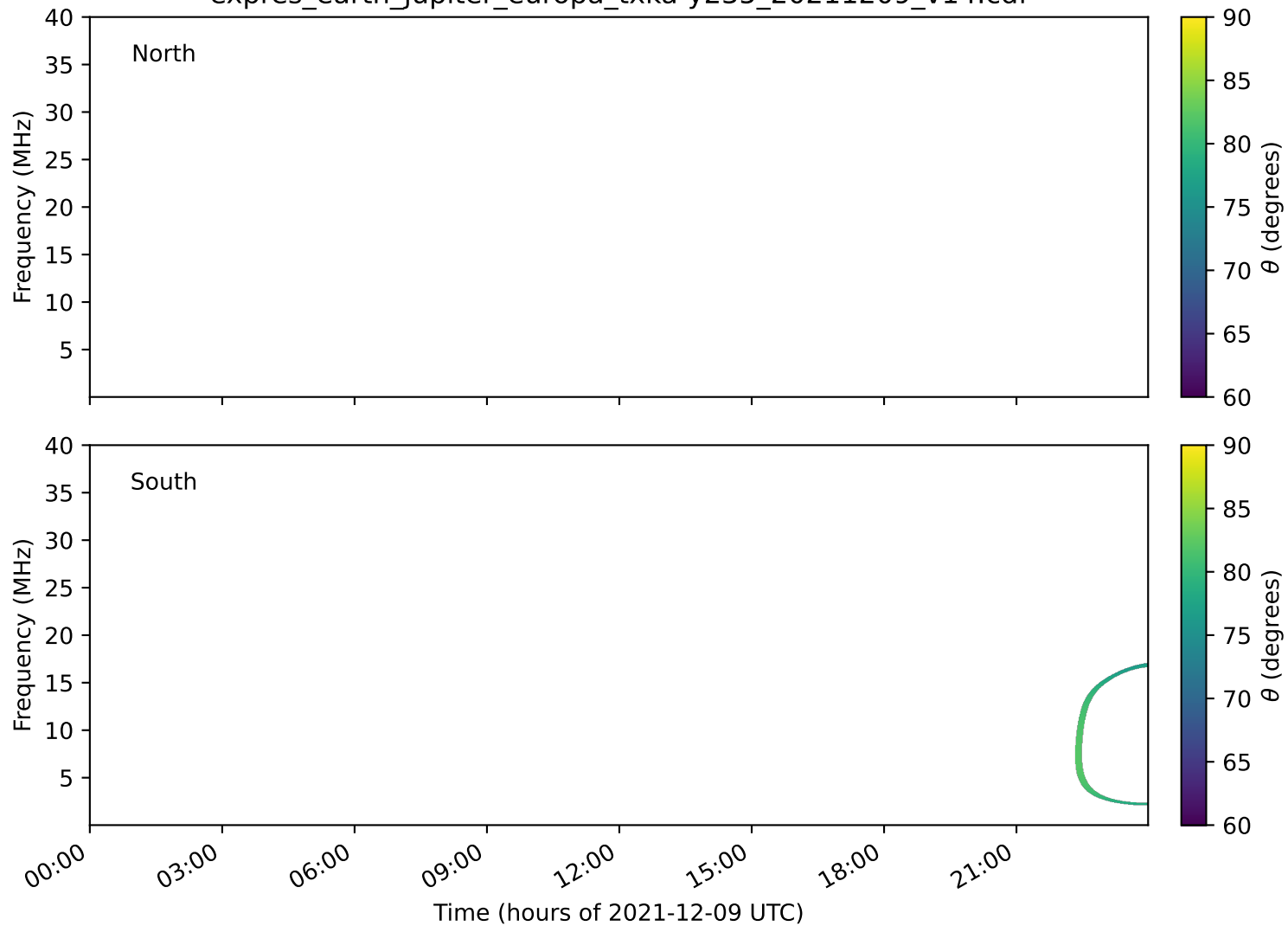
expres_earth_jupiter_europa_txka-y235_20211209_v14.cdf
