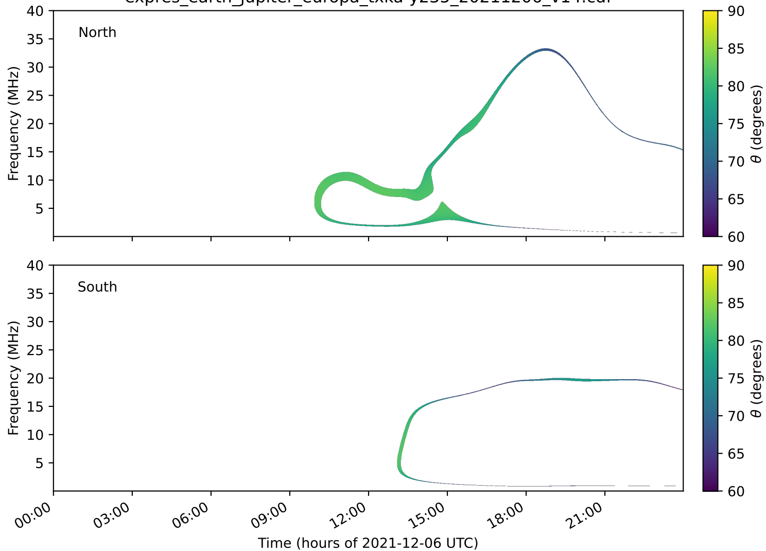
expres_earth_jupiter_europa_txka-y235_20211206_v14.cdf
