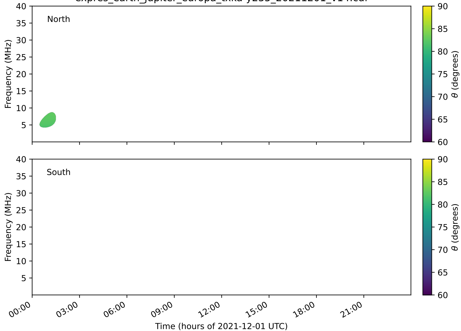
expres_earth_jupiter_europa_txka-y235_20211201_v14.cdf
