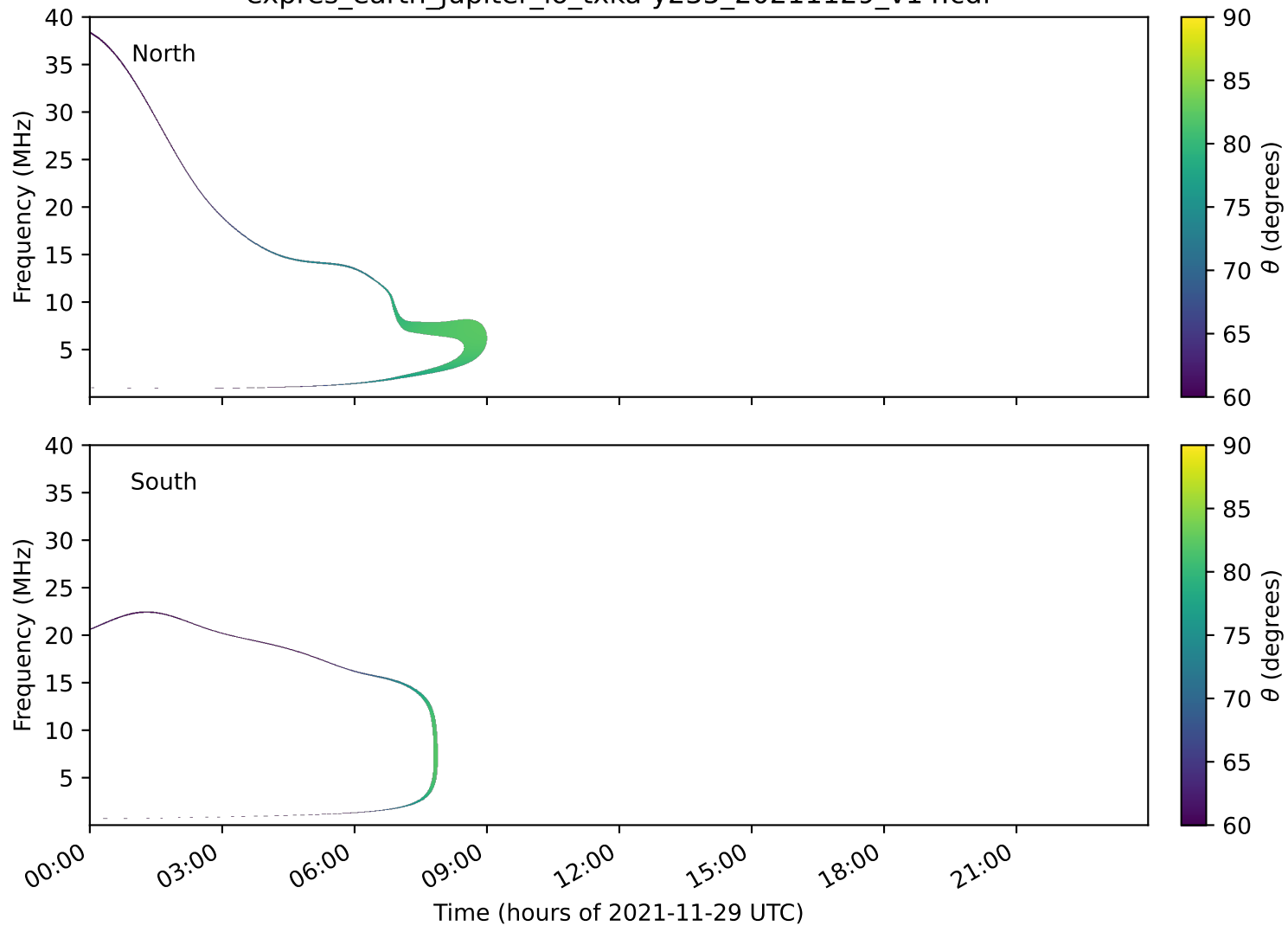
expres_earth_jupiter_io_txka-y235_20211129_v14.cdf
