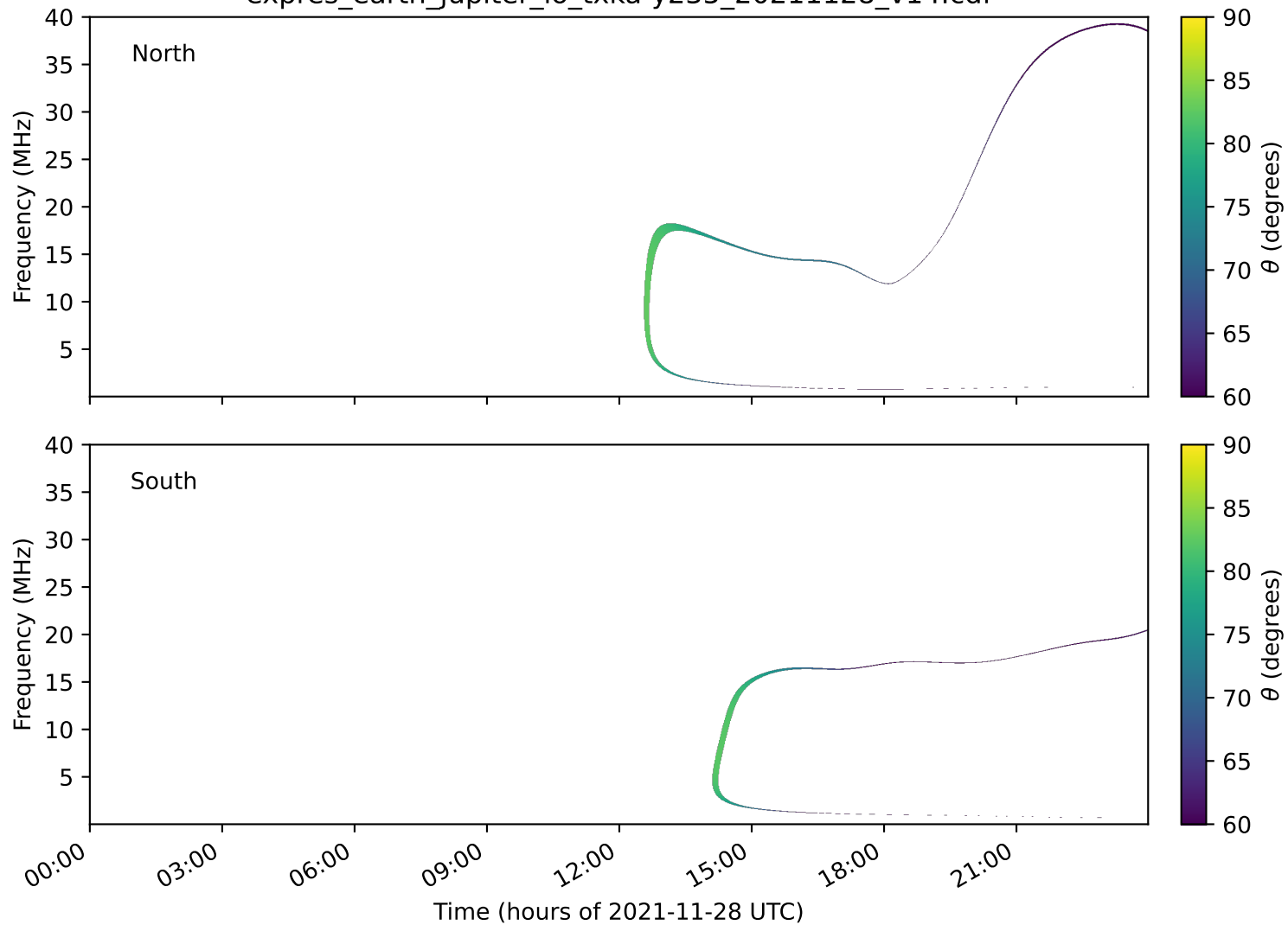
expres_earth_jupiter_io_txka-y235_20211128_v14.cdf
